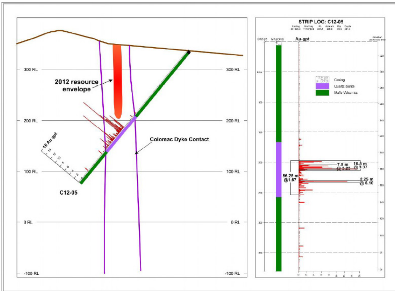
Figure 3 – Hole C12-005 Cross Section and Strip Log
