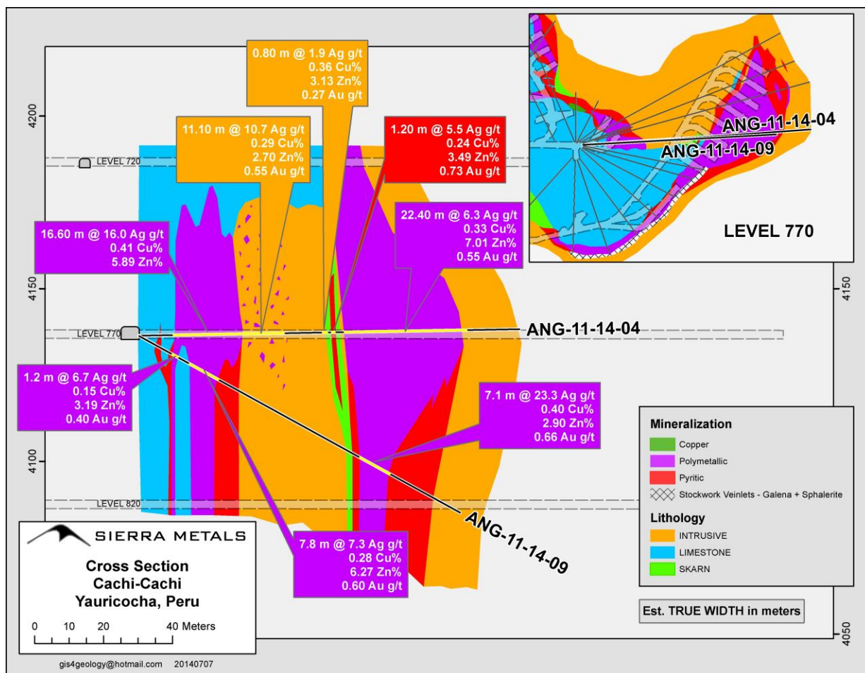
Figure 1: Cross Section along Holes ANG-11-14-04 and -09, and Plan Map of Level 770, Cachi Cachi Mine
