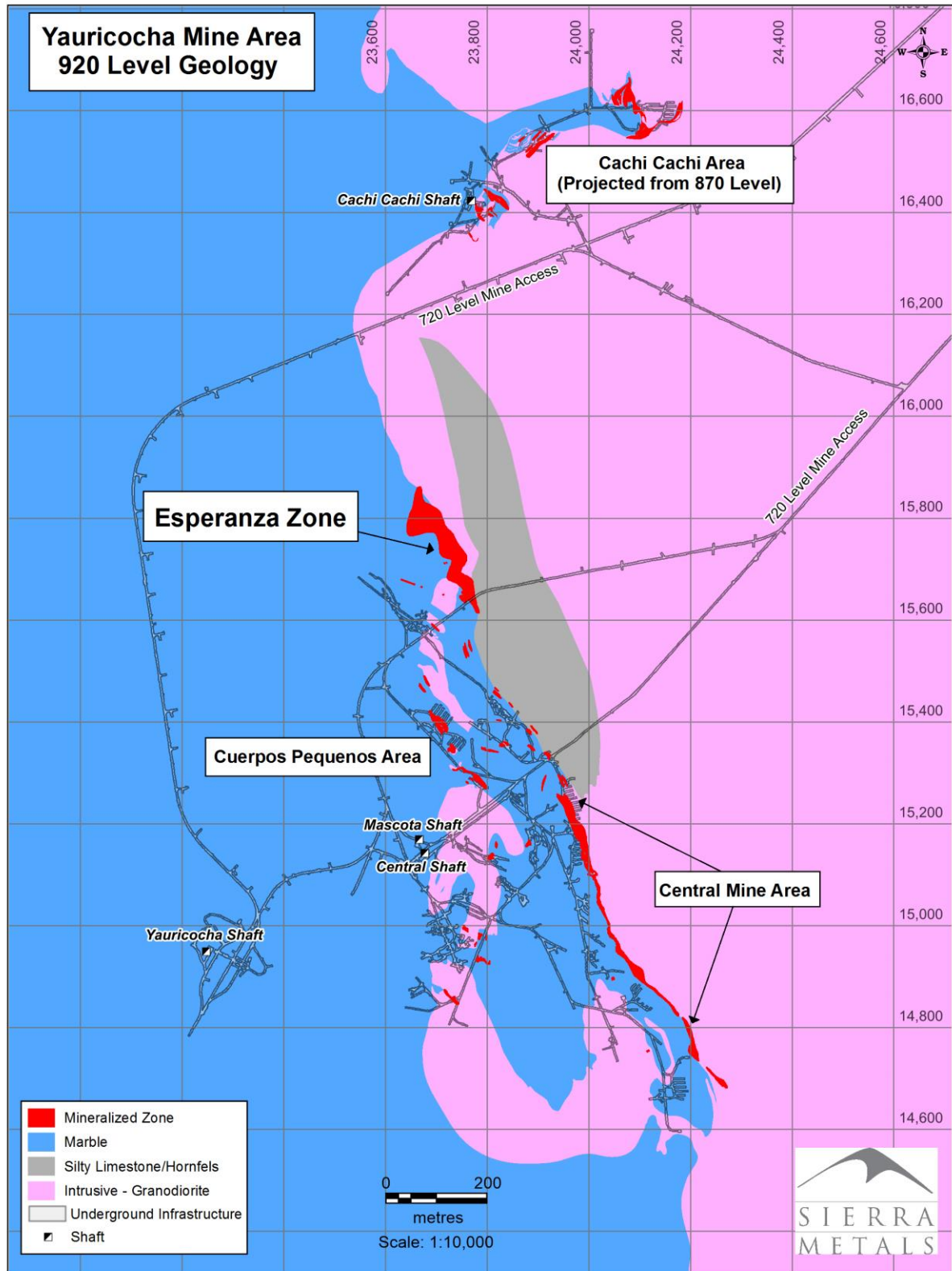
Figure 1 - Plan View
