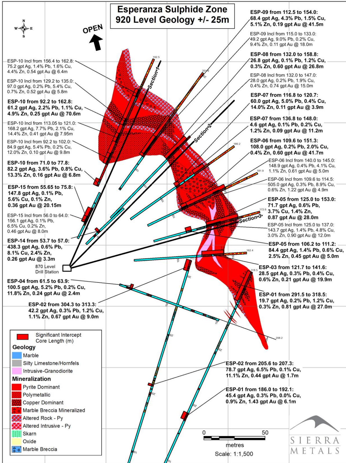
Figure 2 - Plan View
