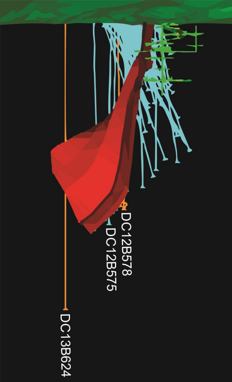
Figure 2: 3D Perspective View of Veta del Contacto
