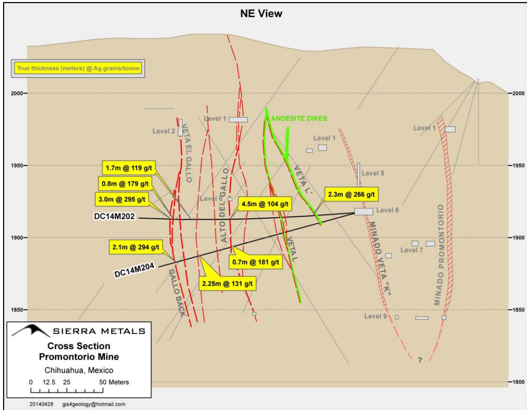
Figure 2: Cross Section along Drill Holes DC14M202 and DC14M204 (note: Section does not cross Azucarera, which is about 100 m NE of section)
