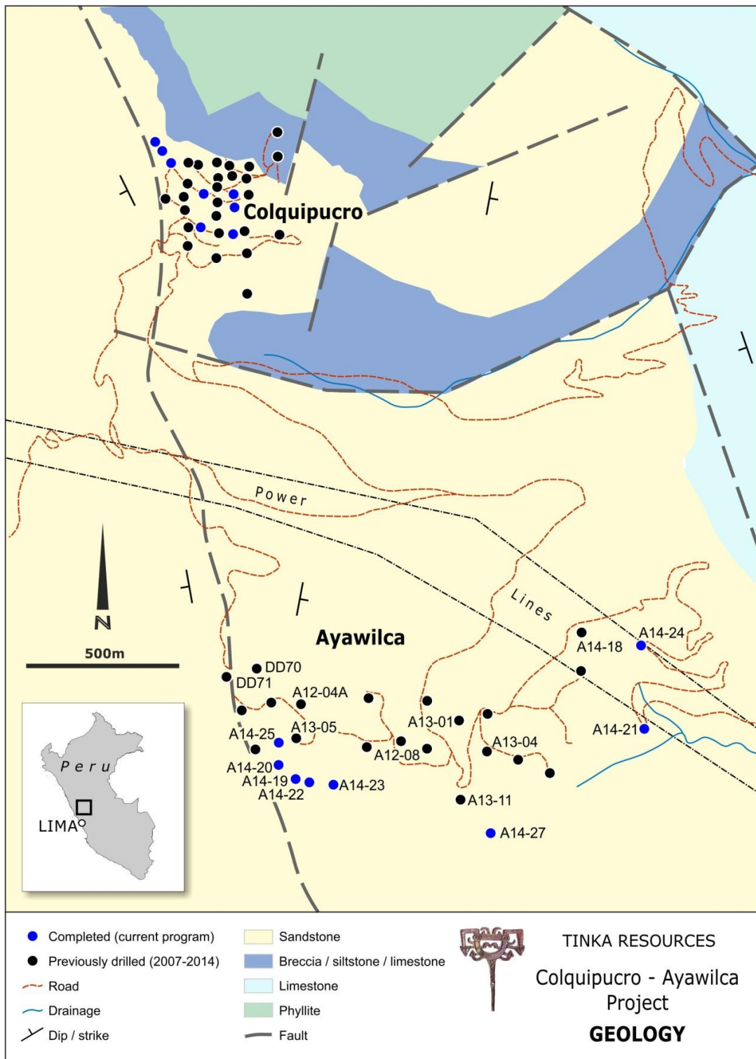
Figure 3. Geology and location map of Aywilca-Colquipucro projects, central Peru
