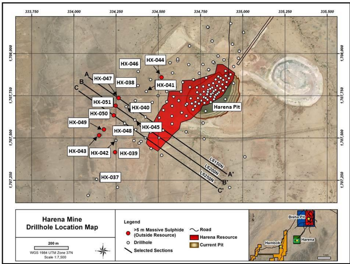
Figure 1. Harena Mine – Drillhole Location Map
