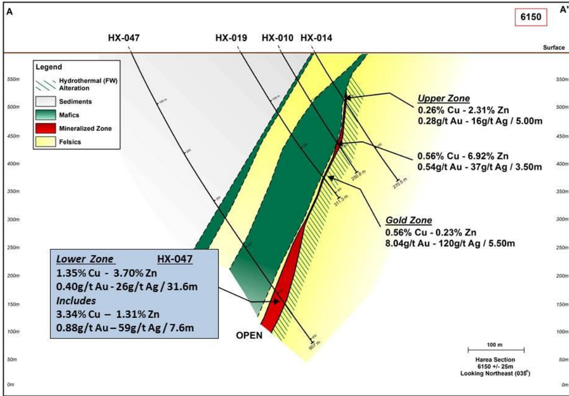
Figure 2. Harena - Section A-A' L6150
