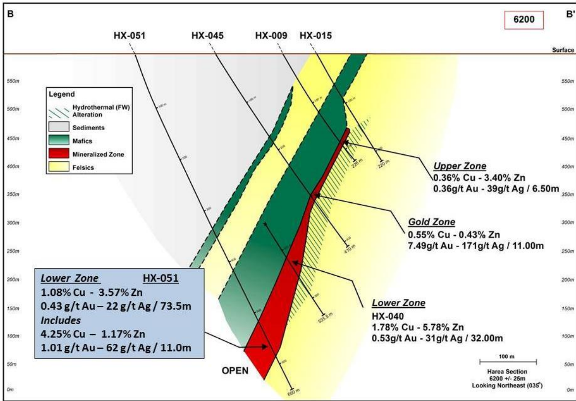
Figure 3. Harena - Section B-B' L6200
