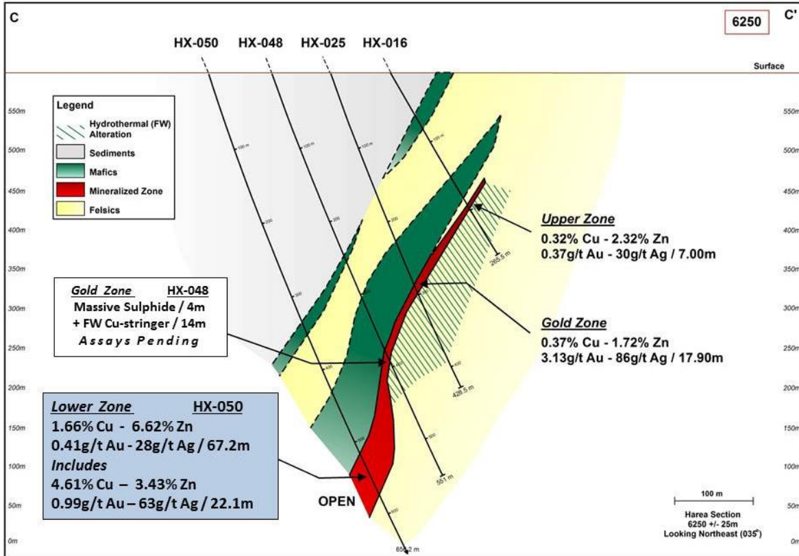
Figure 4. Harena - Section C-C' L6250
