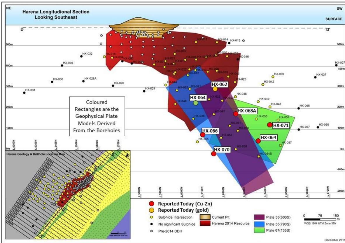
Figure 2. Harena Long Section
