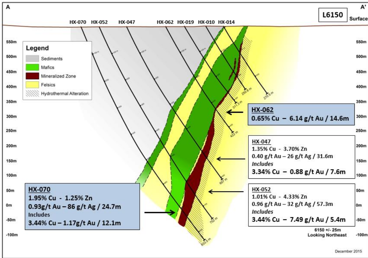
Figure 3. Harena Section L6150
