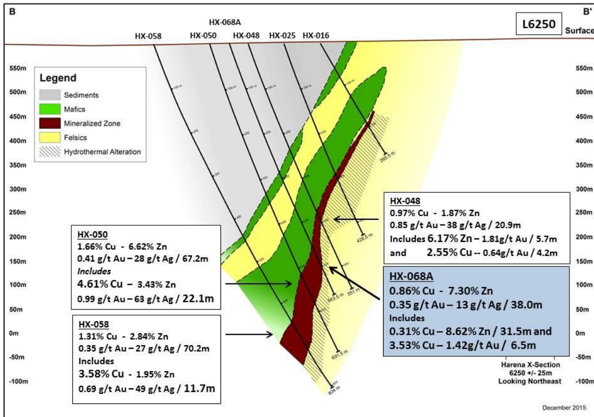
Figure 4. Harena Section L6250
