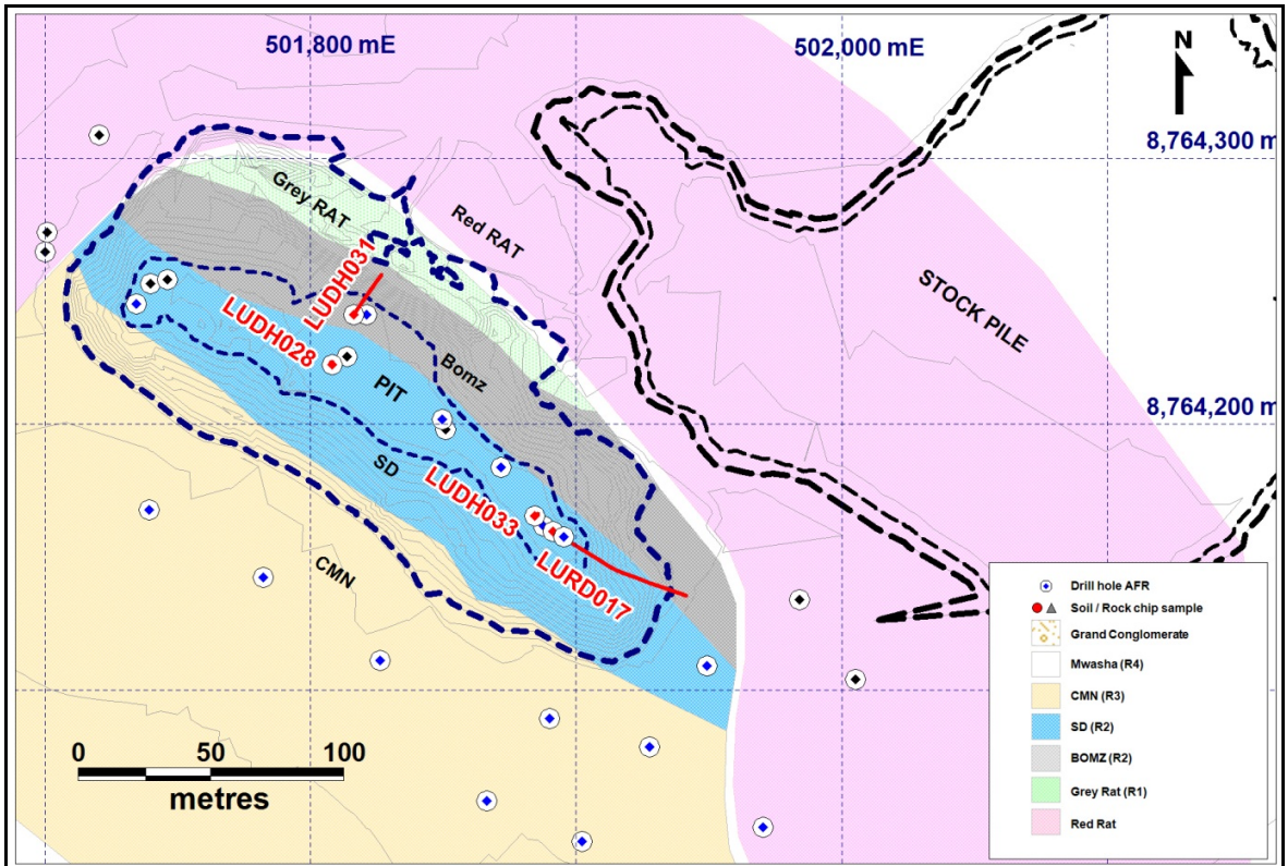
Figure 1: Luisha diamond drill holes (blue); 10 as holes cored from surface and 12 as diamond tails to RC pre-collars; holes with reported assay results are highlighted red (4 in pit; 2 regional).
