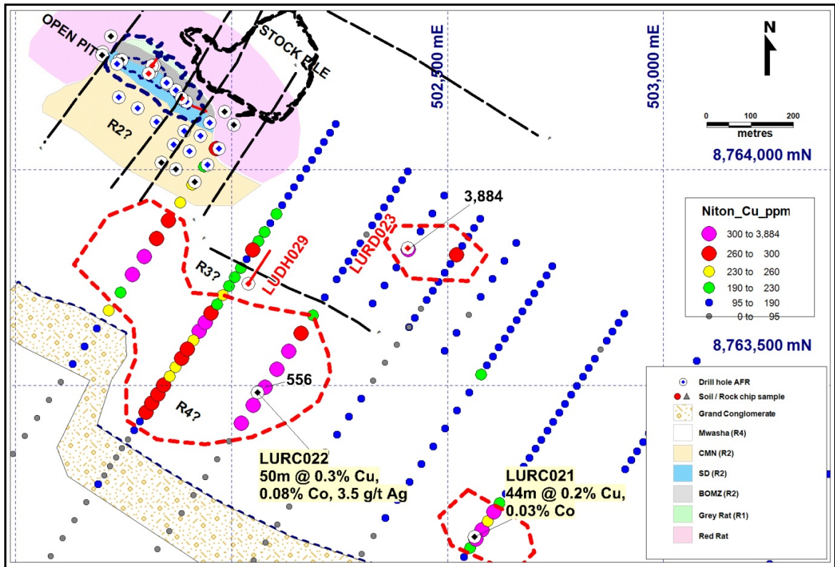
Figure 2: Luisha regional diamond drill holes (red), with regional copper-in-soil geochem anomalies.
