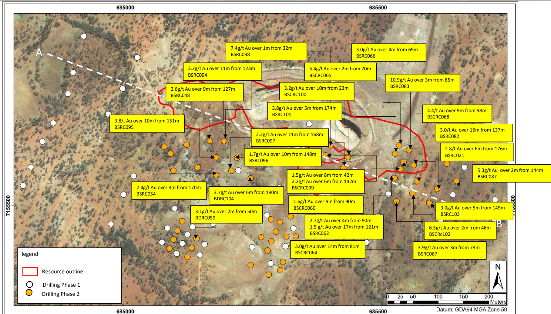
Figure 2 – Drill Plan and Highlighted Intersections
