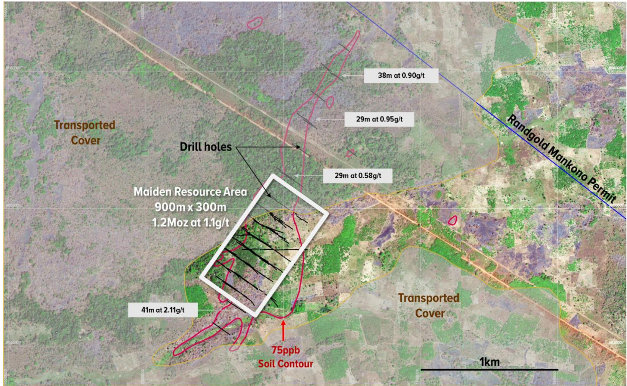
FIGURE 2: Koné Prospect Map (Morondo License)
