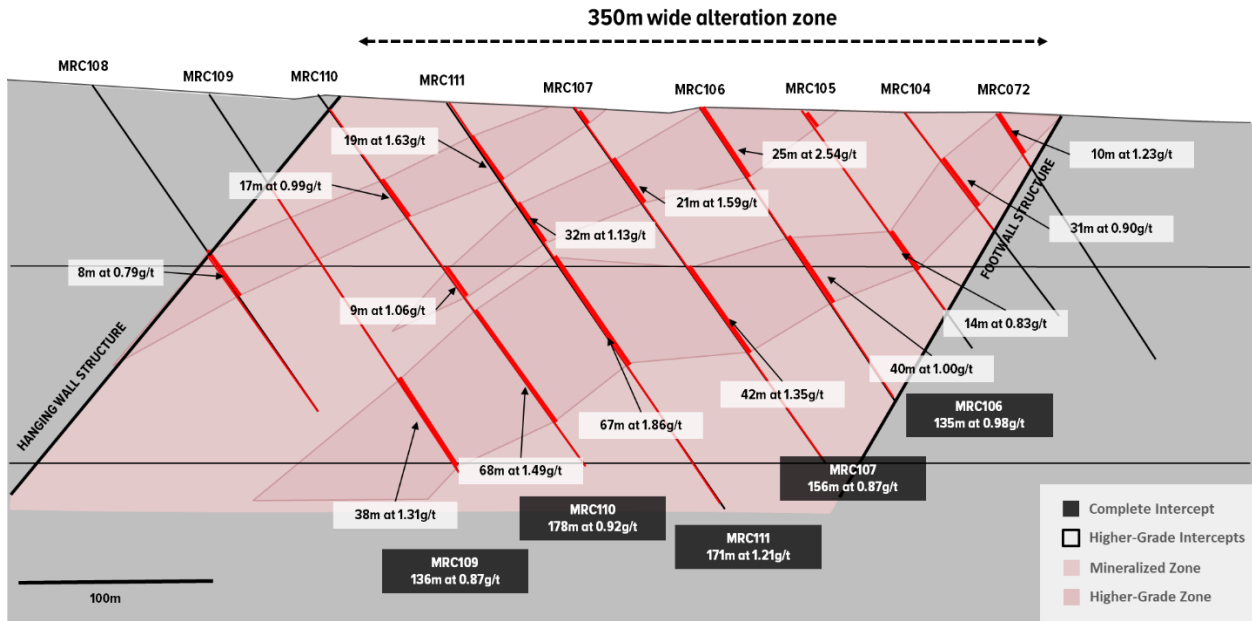
FIGURE 3: Koné Drill Section
