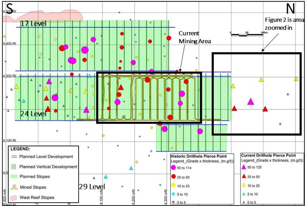
Figure 1: Prestea Underground Longsection
