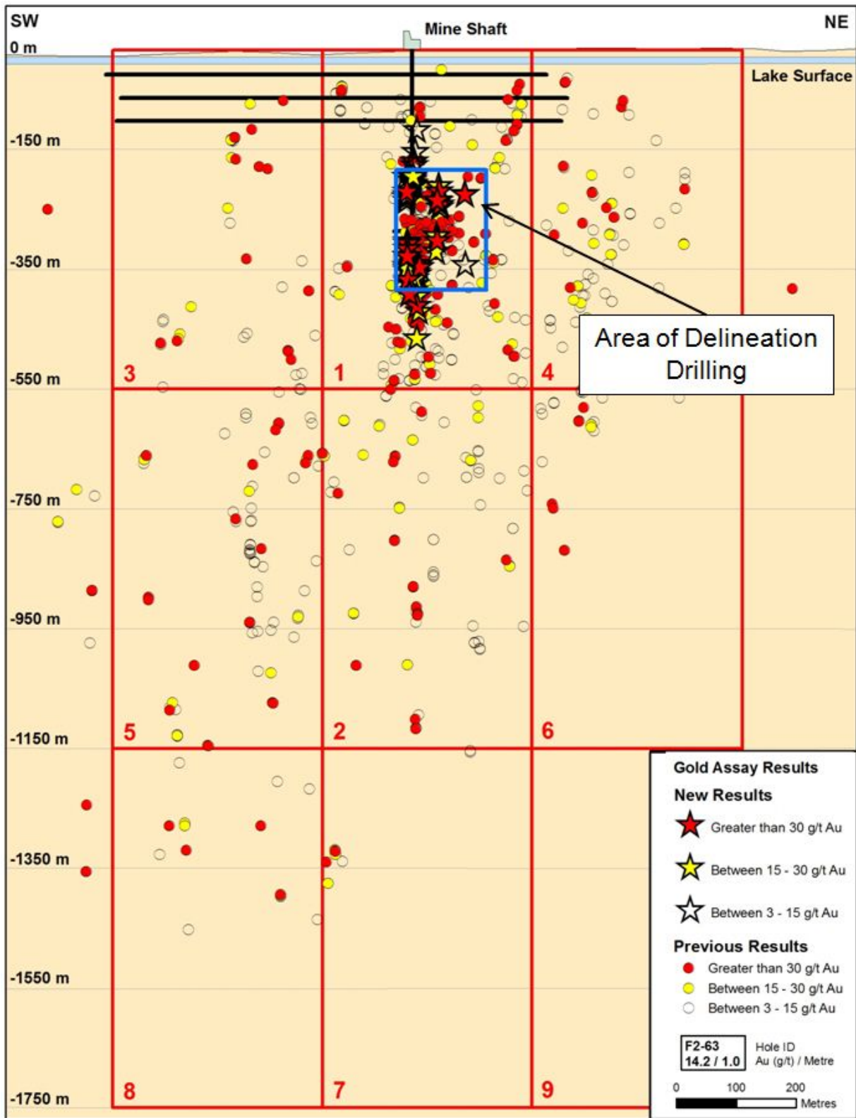
Figure 4: F2 Gold System composite long section showing area of delineation drilling
