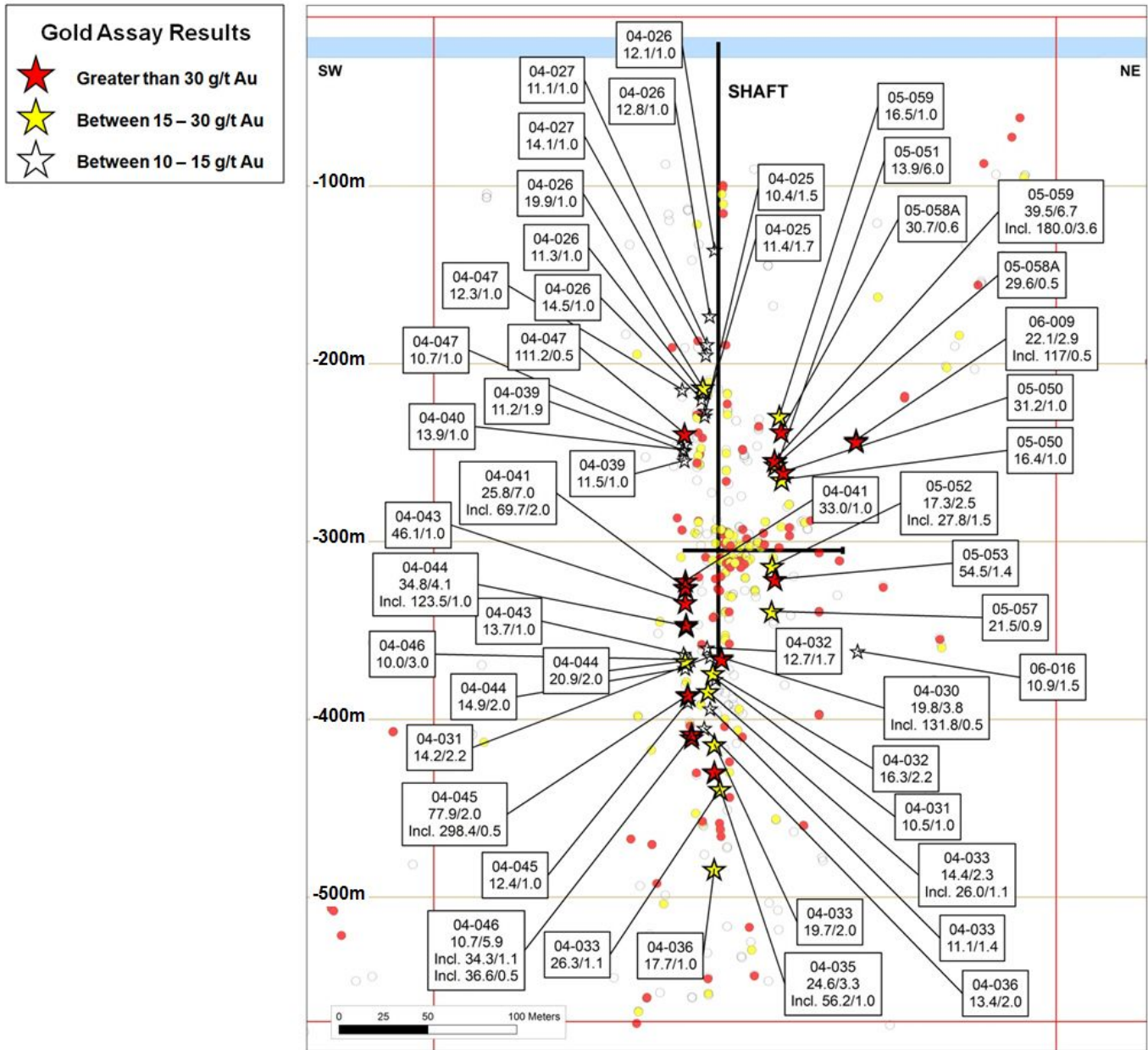
Figure 5: Detailed long section showing delineation drilling results >10 g/t gold
