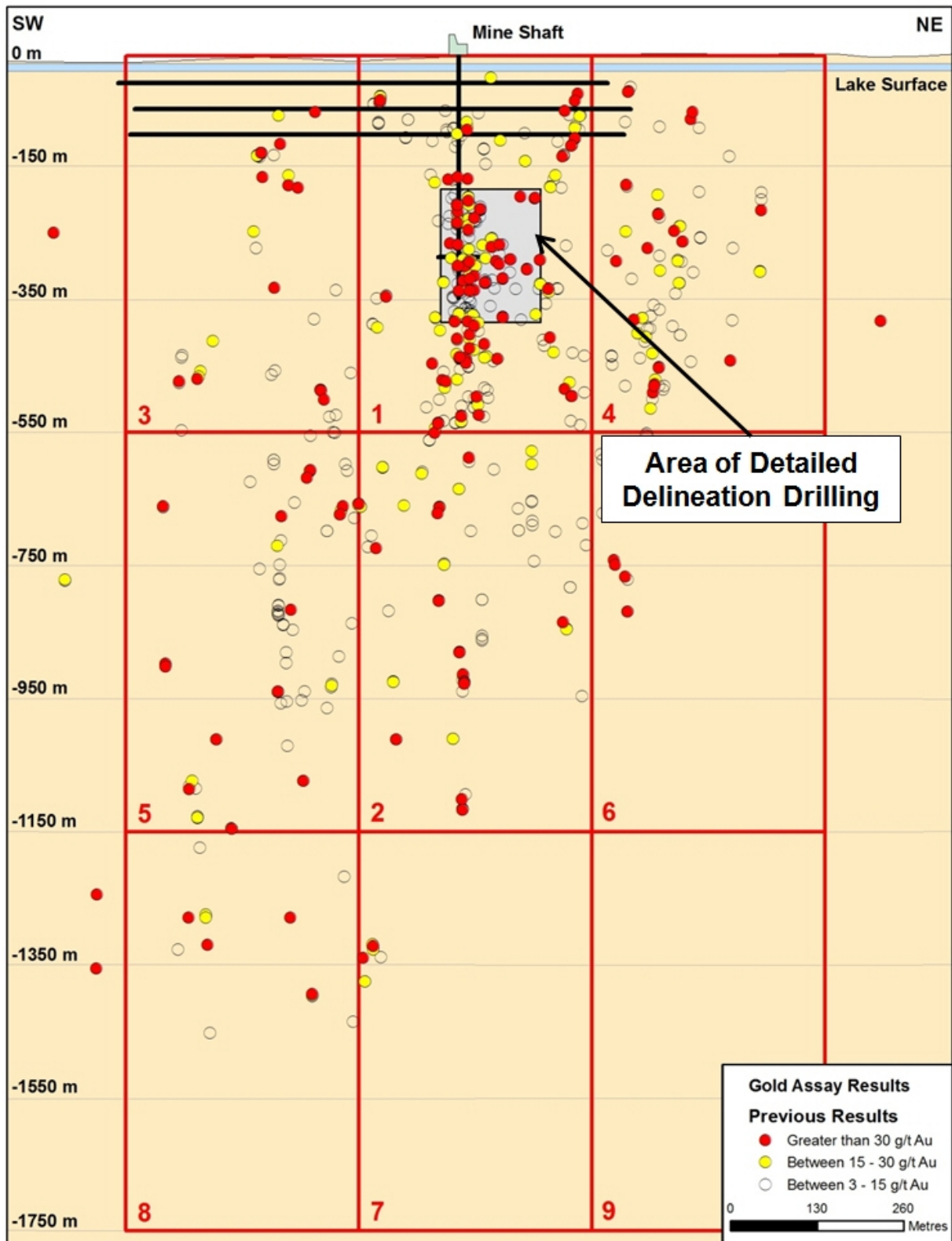
Figure 5: Composite Long Section Looking Northwest and 9X Target
