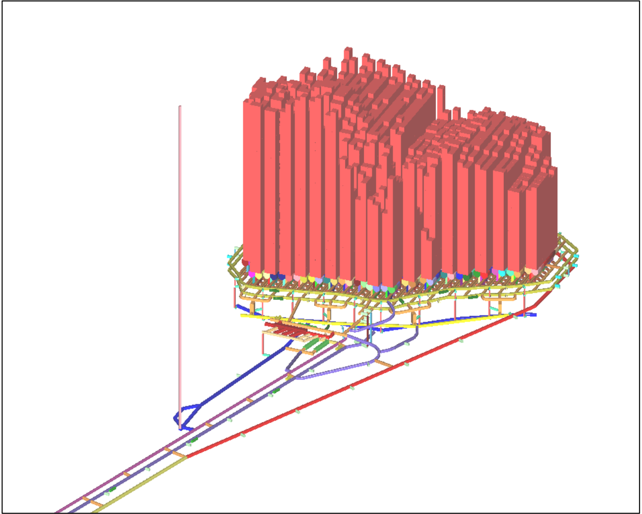
Appendix 3: Isometric view of KUG mine workings and cave (red)
