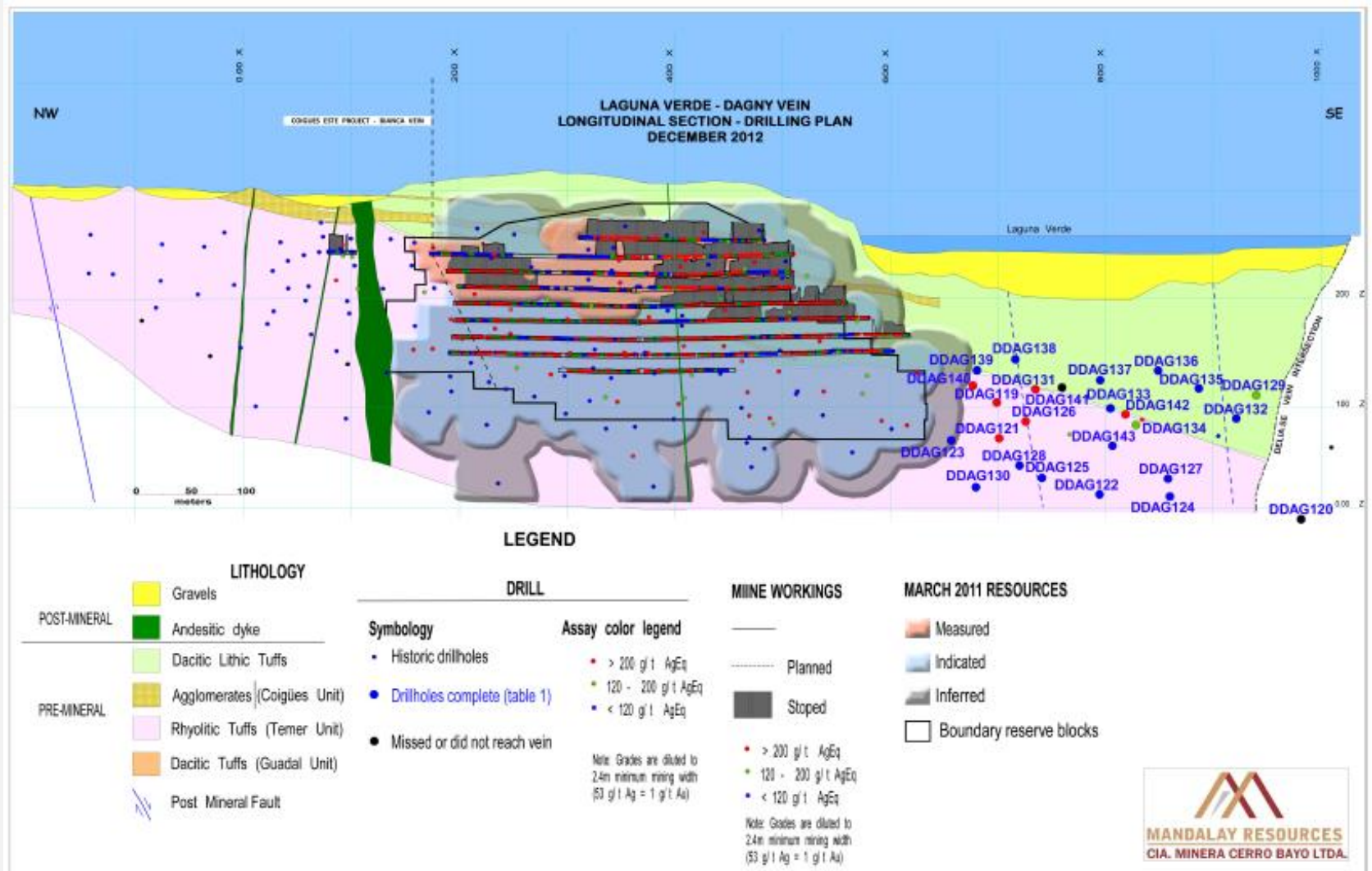
Figure 2: Dagny Long Section
