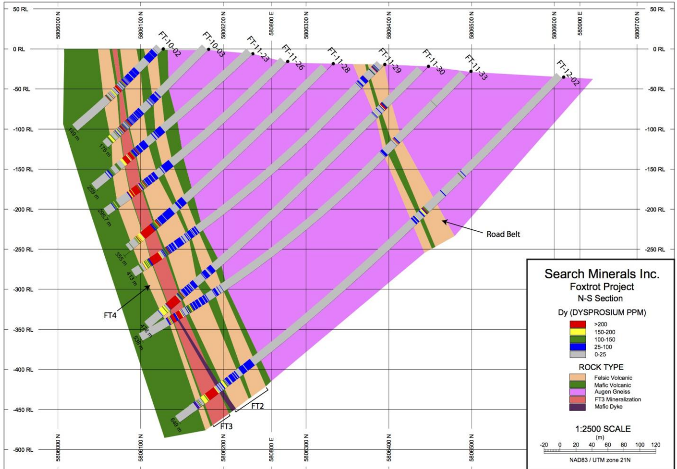
Figure 4 - Foxtrot Project Representative North-South Dy and Geology Cross Section
