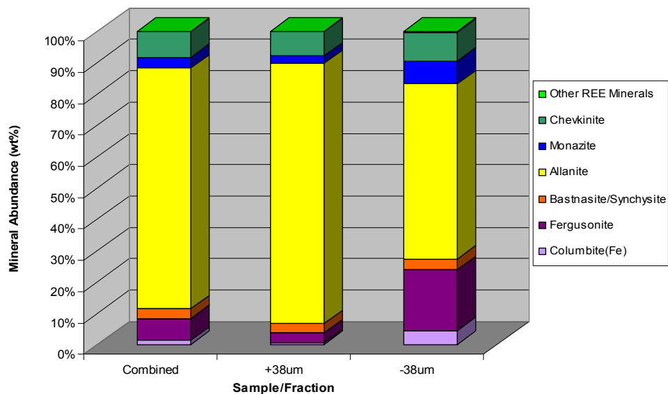
Figure 1 – Normalized Mineral Abundance of REE Minerals
