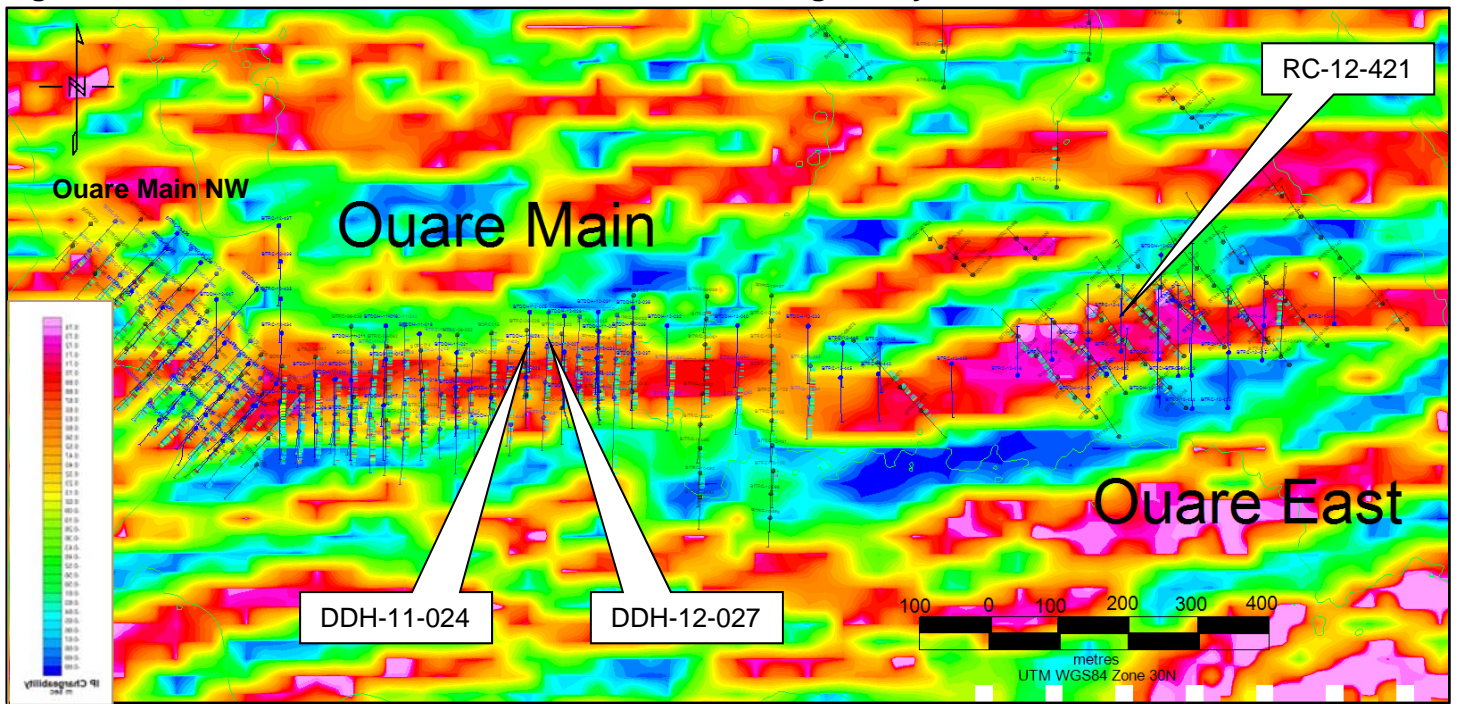
Figure 3: Ouare Main and Ouare East Drill Plan on IP Chargeability
