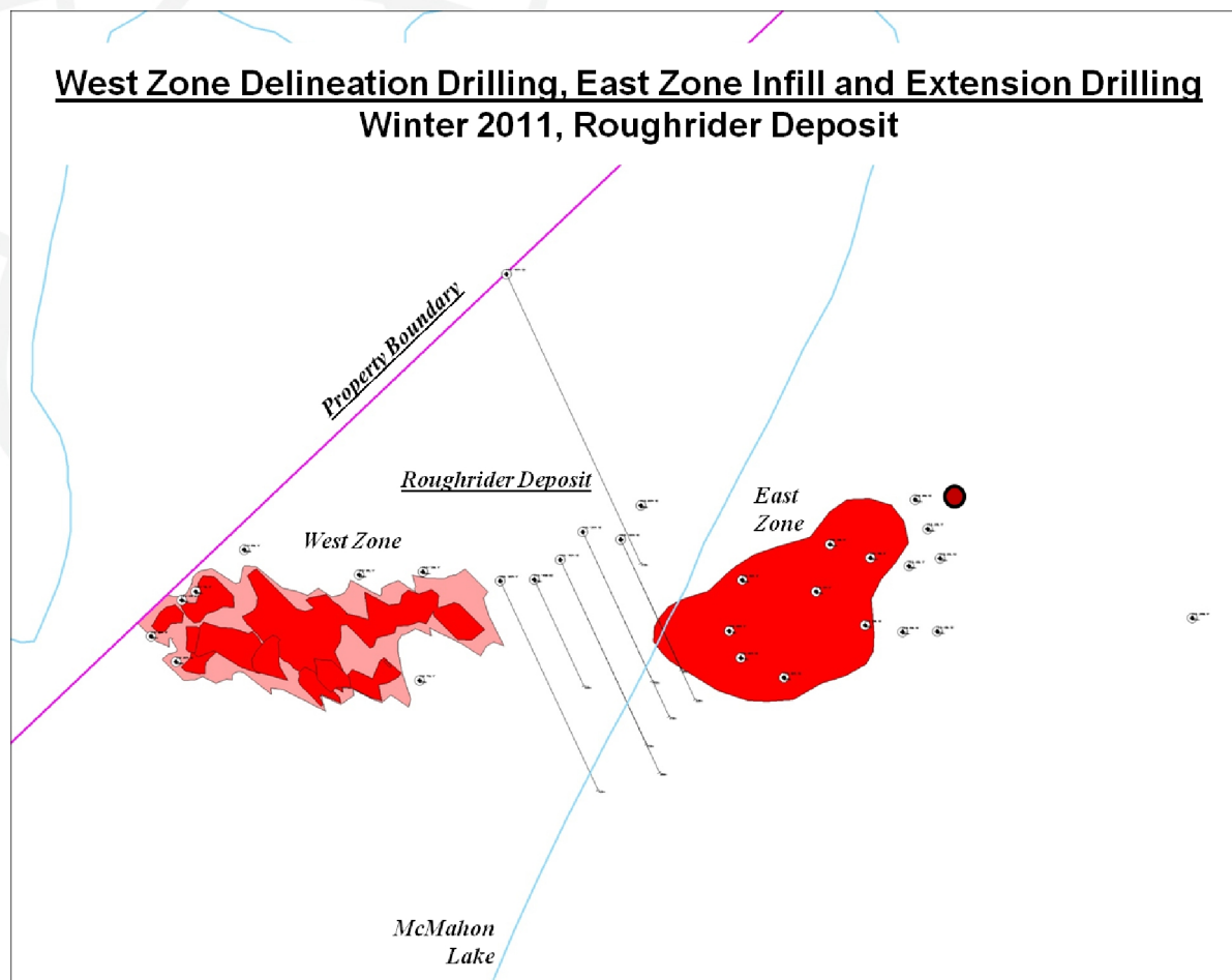
Figure 1. Location map for drill holes planned for 2011 winter season, Roughrider Project (see news Release dated January 20, 2011). Outline of East Zone encompasses 2010 drill holes with uranium mineralization between L 100 W and 60 E (160 m strike). Red circle is new mineralization in hole MWNE-11-667 on L 100E.
