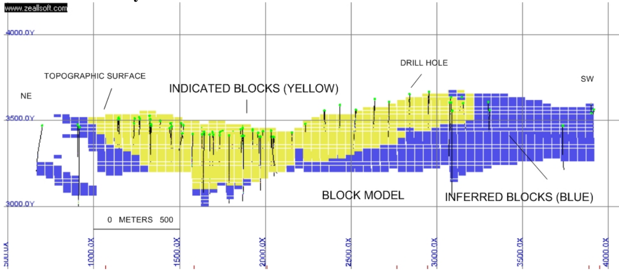
SAWAYERDUN ZONE IV BLOCK MODEL LONG SECTION LOOKING SOUTHEAST
