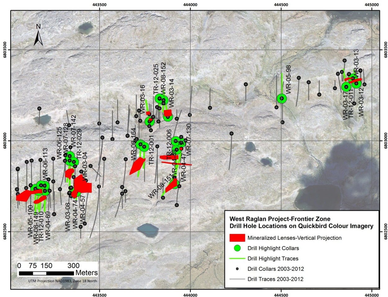
Figure 2: Key map for the significant mineralized drill intersections included in Table 1. Source: True North Nickel
