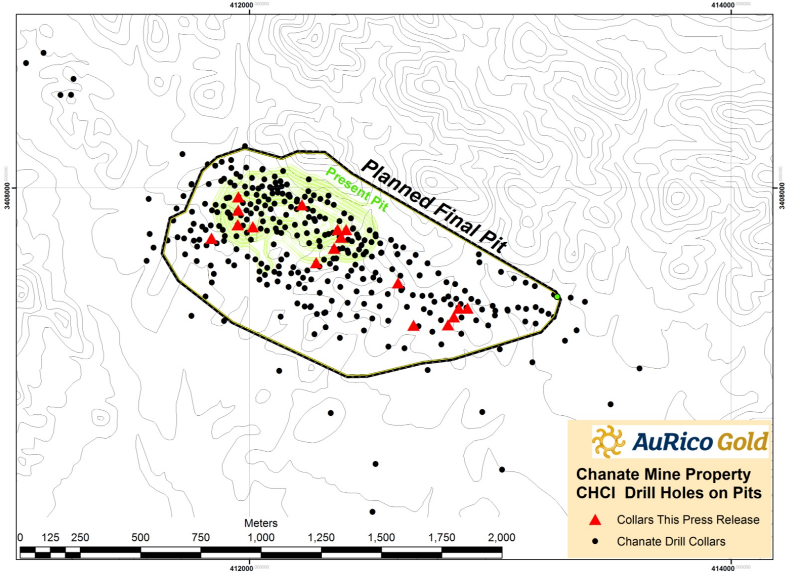
Diagram 1: El Chanate Plan Map
