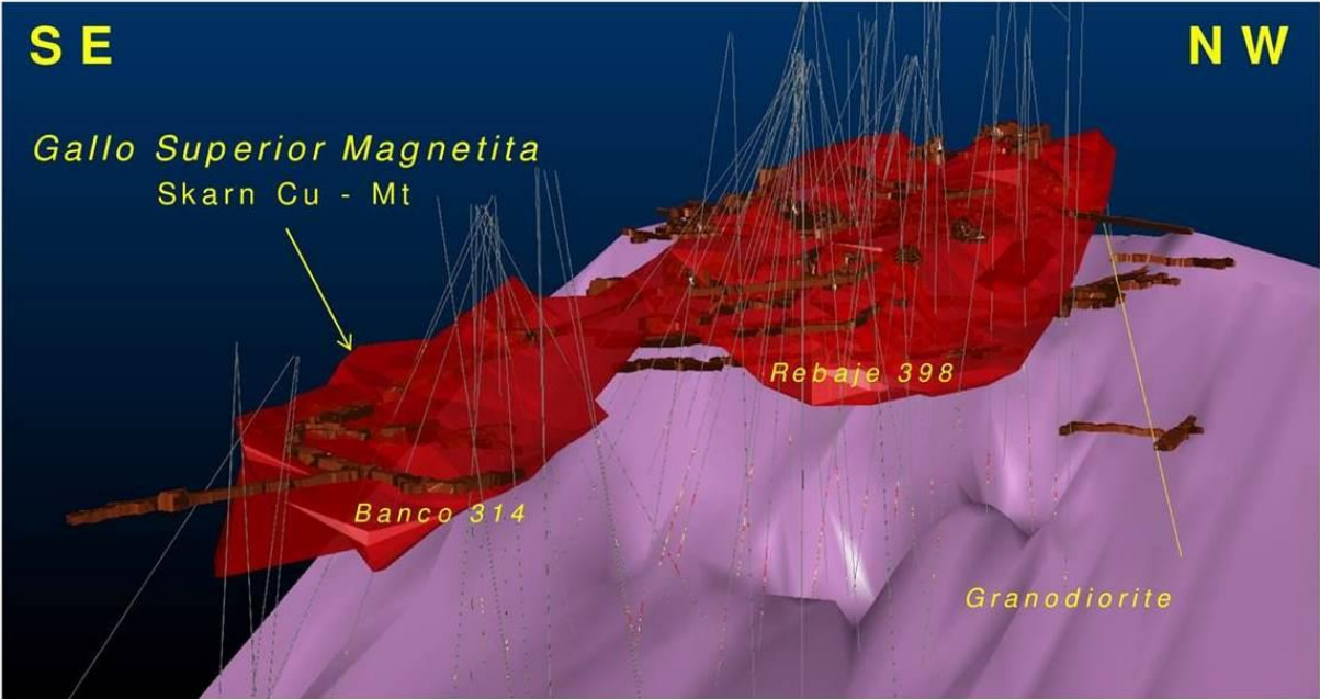
Figure 1: Perspective View to SW of Gallo Superior Magnetita of the Upper Skarn Horizon, Bolivar Mine
