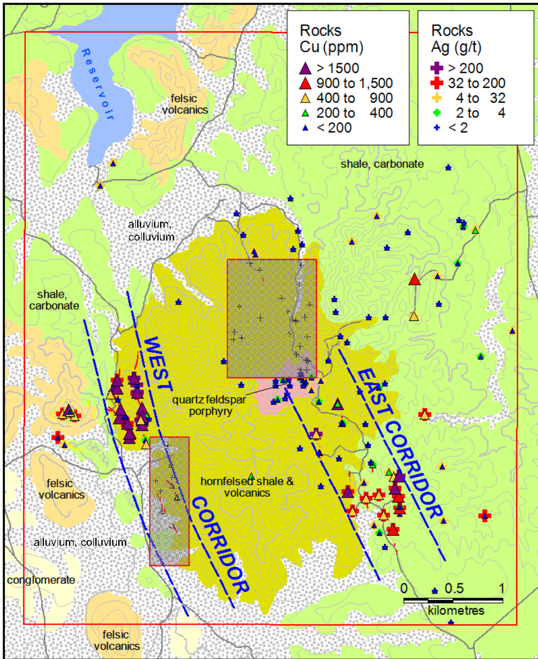
Figure 2: Valsequillo Geology and Sampling Results; greyed areas are 3 rd party concessions.
