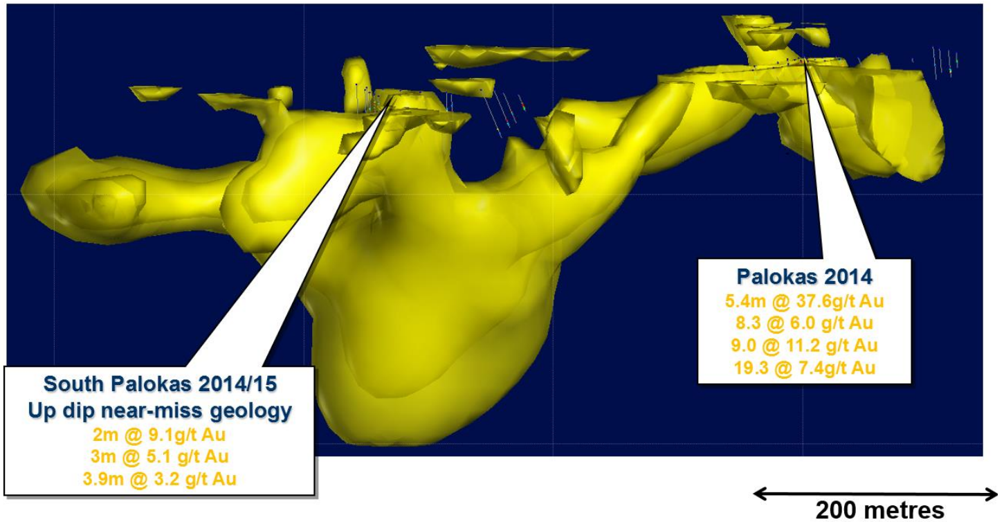
Figure 1: 3D IP Resistivity Shells (2.0 to 2.5 (log[Ohm-m]) from Palokas to South Palokas showing 600 metre strike length low resistive/conductor. Conductor correlates with drilling at Palokas and plunges below drilling at South Palokas.
